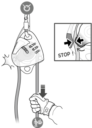
Locking Blocage
