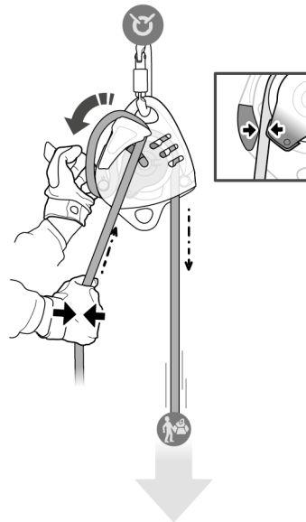
Lowering Descente
