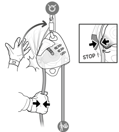
AUTO-LOCK system Système AUTO-LOCK
